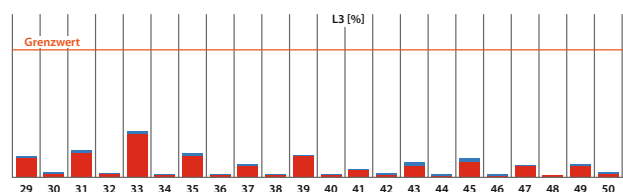
Harmonics with high pass filter
